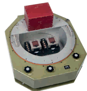
Example of Wild/Leica mount with mount adapter, IMU and two digital cameras.
